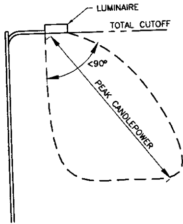
CUTOFF LUMINAIRE WITH LESS THAN 90° CUTOFF
