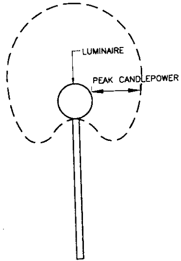
NO CUTOFF LUMINAIRE
