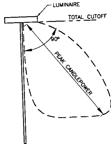
CUTOFF LUMINAIRE
